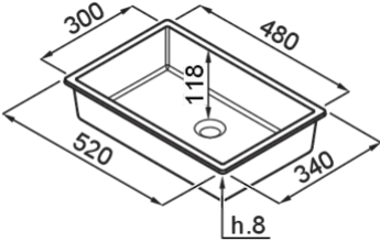
Technical Drawing
