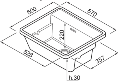
Technical Drawing
