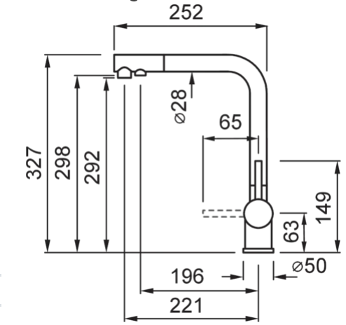
Technical Drawing
