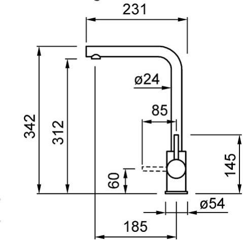
Technical Drawing
